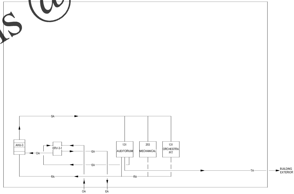
AHU-3 AIR FLOW DIAGRAM
