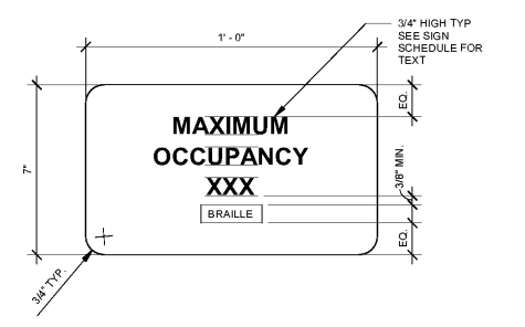
MAXIMUM OCCUPANCY SIGN - (S6) ⑥ 3" = 1'-0"
