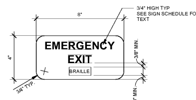
EMERGENCY EXIT SIGN - (S4) ④ 3" = 1'-0"
