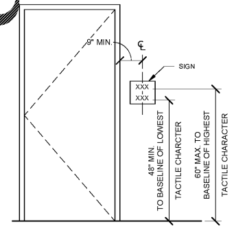
SIGNAGE HEIGHT DETAIL ⑦ 1/2" = 1'-0"
