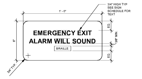
EMERGENCY EXIT WITH ALARM - (S5) ⑤ 3" = 1'-0"
