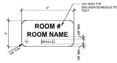
DOUBLE LINE TEXT SIGN - (S2) ② 3" = 1'-0"
