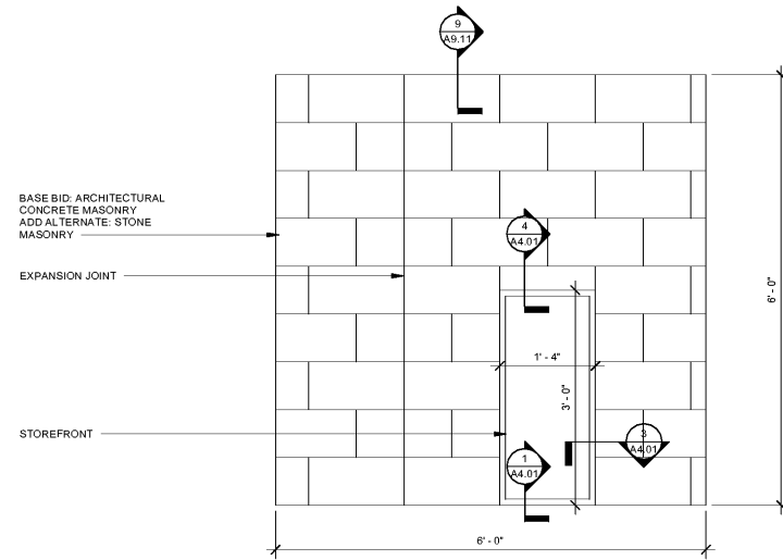
MOCK UP 2 3/4" = 1'-0" ②
