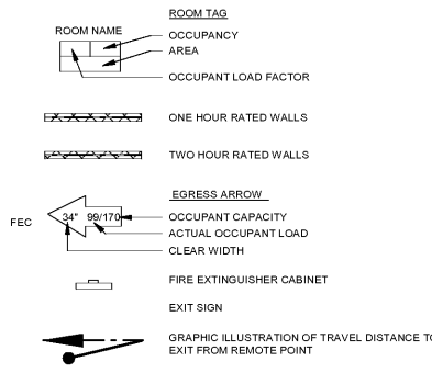
LIFE SAFETY LEGEND 1/8" = 1'-0"
