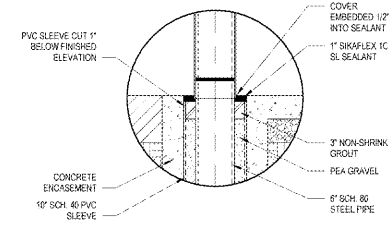
11 ENLARGED BOLLARD DETAIL CA2 1" x 1'-0"
