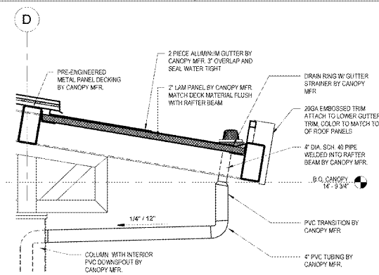
18 SECTION @ TRENCH DRAIN CA2 3/4" x 1'-0"
