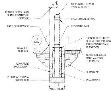
5 BOLLARD DETAIL CA2 12" x 1'-0"
