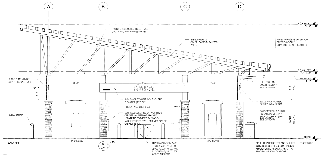
27 CANOPY ELEVATION CA2 1/4" x 11'-0"
