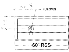
60" RSS PLAN VIEW
