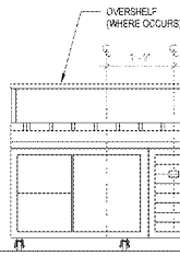
REFRIGERATED SANDWICH STATION ELEVATION VIEW
