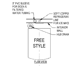
FREE STYLE PLAN VIEW
