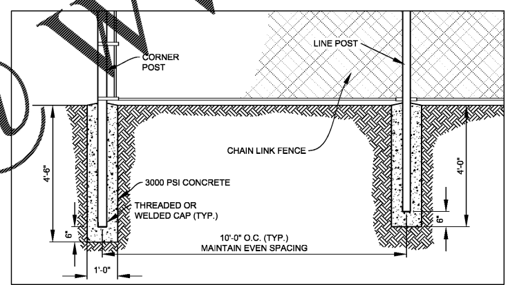
BATTING CAGE FOOTERS
