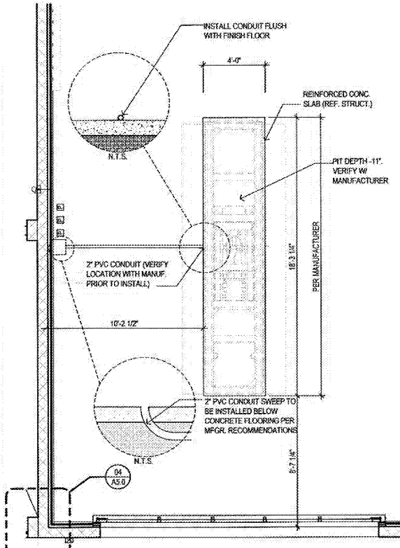
04 PLAN DETAIL (FRAME RACK PIT) 1/4"=1'-0"
