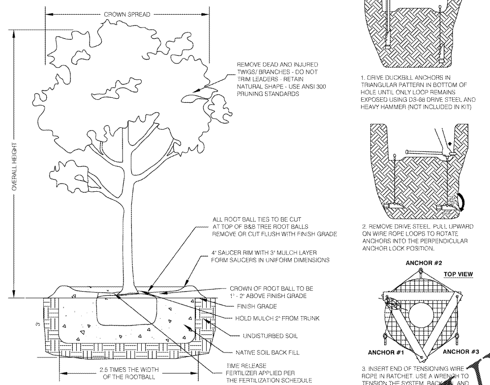
1 LARGE TREE PLANTING DETAIL (3" OR GREATER CALIPER) LS3 NOT TO SCALE
