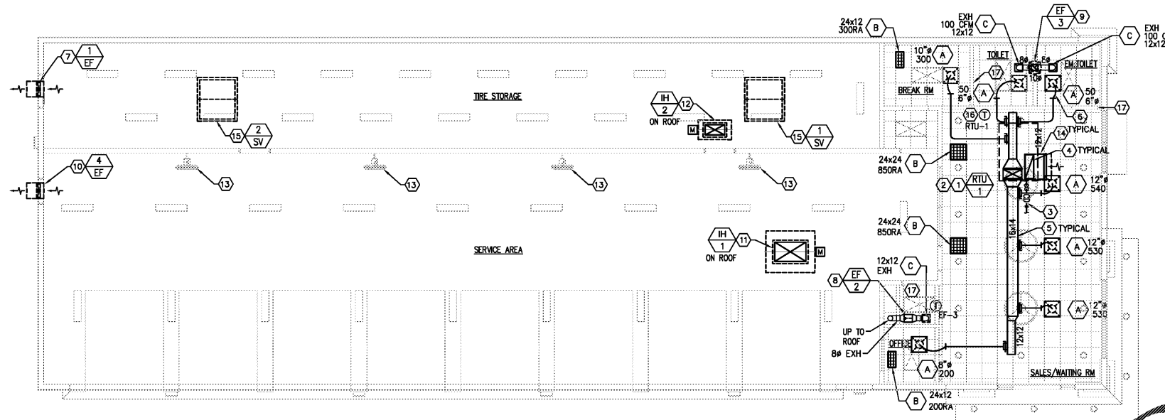
1 MECHANICAL PLAN 1/8" = 1'-0"
