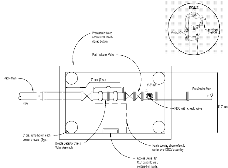
Fire Department Vault Plan View
