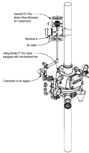
Dry Valve and Riser-Mounted Air Compressor Detail (Porte Cochere)
