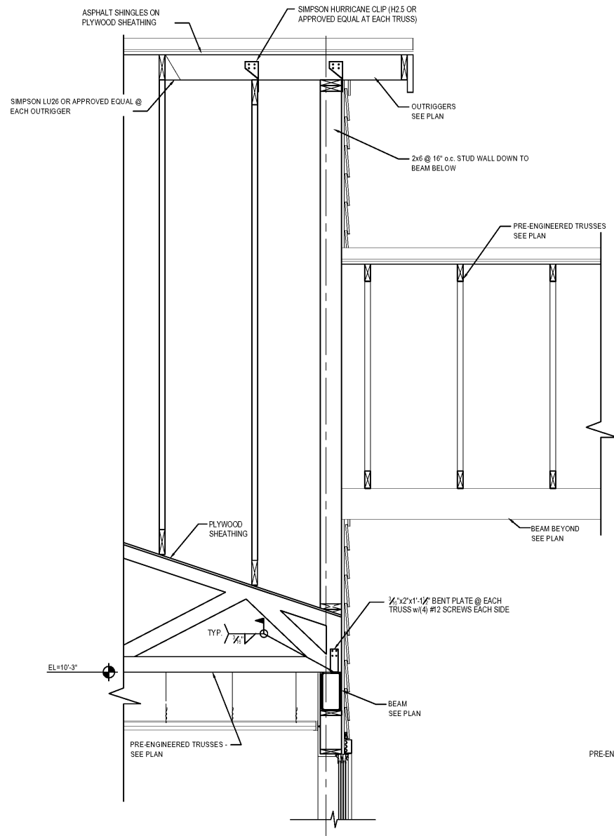
1 SECTION 3/4" = 1'-0" S5.1 | S6.2
