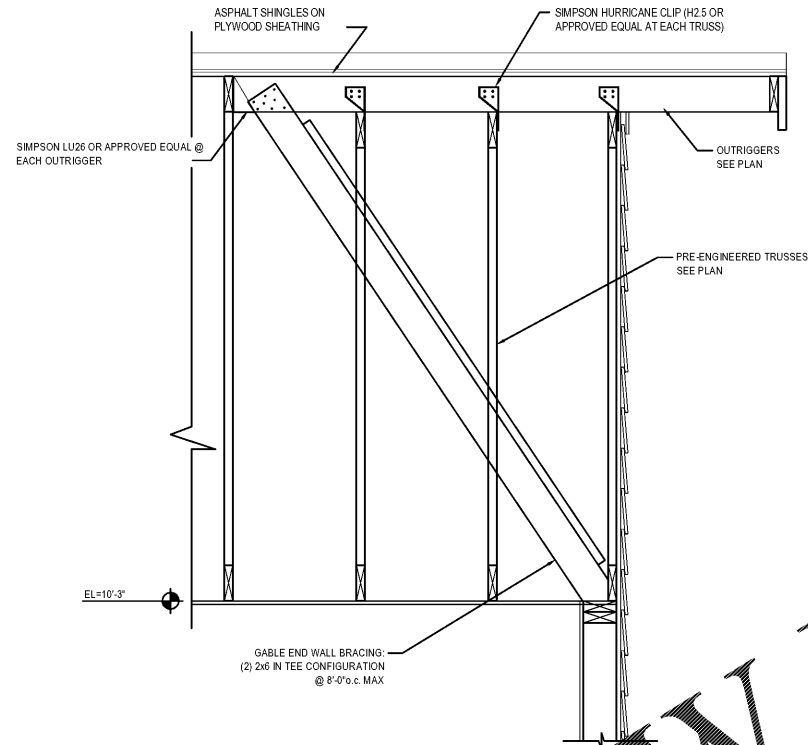
2 SECTION 3/4" = 1'-0" S5.1 | S6.2
