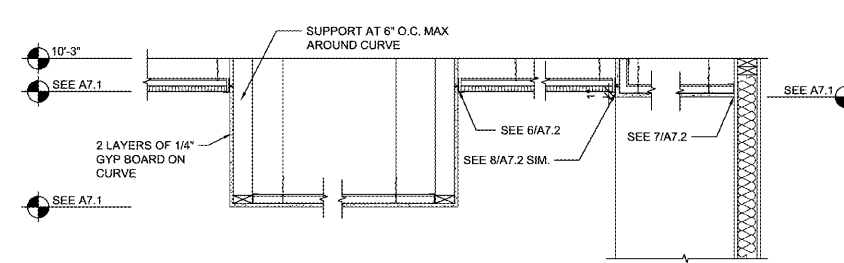
3 CEILING SECTION SCALE: 3/4" = 1'-0" AT MEDICAL NURSES STATIONS
