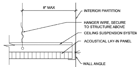
6 TYPICAL DETAIL SCALE: 3" = 1'-0"
