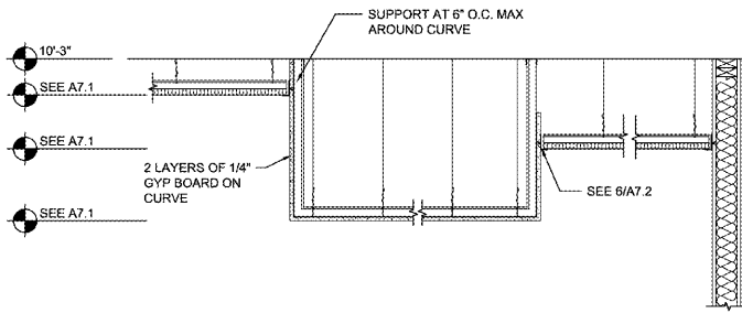
4 CEILING SECTION SCALE: 3/4" = 1'-0" AT DENTAL RECEPTION
