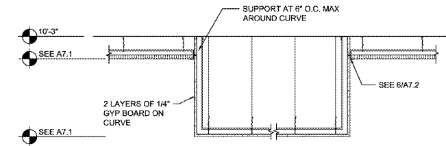
2 CEILING SECTION SCALE: 3/4" = 1'-0" AT DROP SOFFITS
