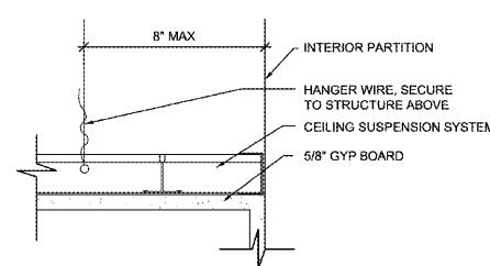
7 TYPICAL DETAIL SCALE: 3" = 1'-0"
