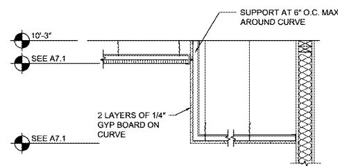
2 CEILING SECTION SCALE: 3/4" = 1'-0" AT DROP SOFFITS
