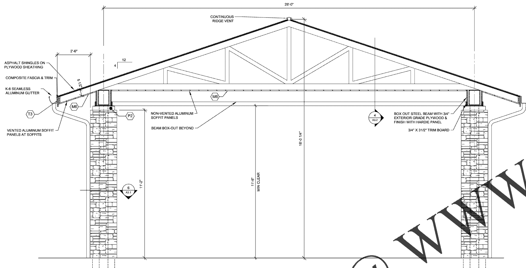
1 CANOPY SECTION SCALE: 1/2" = 1'-0"
