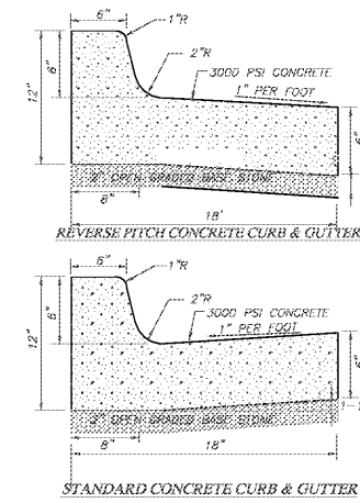
9 C7.0 DETAIL: 1" CONCRETE CURB & GUTTER (NTS)
