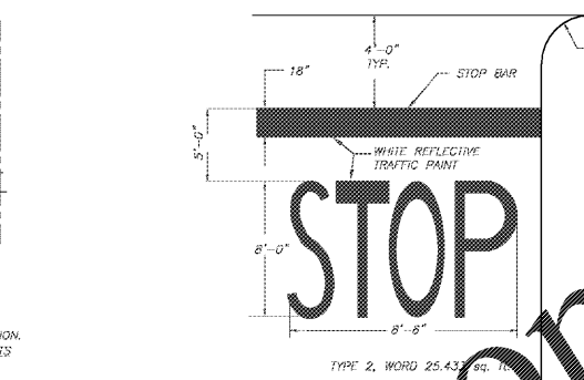
14 C7.0 DETAIL: STOP BAR PAVEMENT MARKING (NTS)
