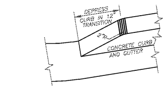
8 C7.0 DETAIL: CURB & GUTTER TAPER OR TRANSITION (NTS)
