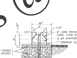
11 C7.0 DETAIL: PRE-CAST CONC. CURB STOP DETAIL (NTS)
