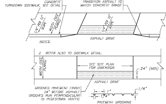
8 C7.0 DETAIL: FLUSH SIDEWALK TRANSITION (NTS)
