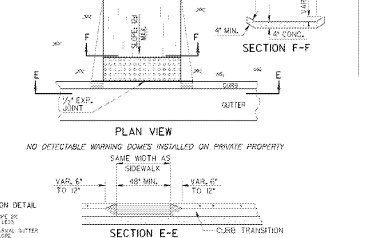
15 C7.0 DETAIL: CURB RAMPS (NTS) TAKEN FROM GDDI STANDARD A3 DATED 9-15-16
