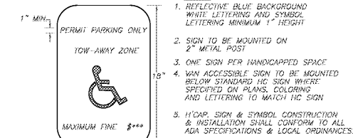
3 C7.0 DETAIL: HANDICAPPED SIGN & SYMBOL (NTS)
