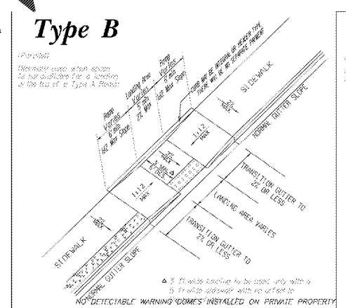
15 C7.0 DETAIL: CURB RAMPS (NTS) TAKEN FROM GDDI STANDARD A3 DATED 9-15-16
