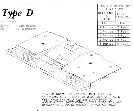
15 C7.0 DETAIL: CURB RAMPS (NTS) TAKEN FROM GDDI STANDARD A3 DATED 9-15-16
