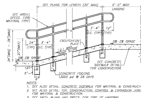
13 C7.0 DETAIL: ACCESSIBLE RAMP WITH HANDRAIL (NTS)
