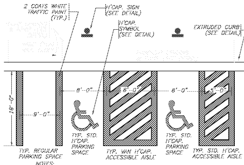
2 C7.0 DETAIL: 90° PARKING (NTS)
