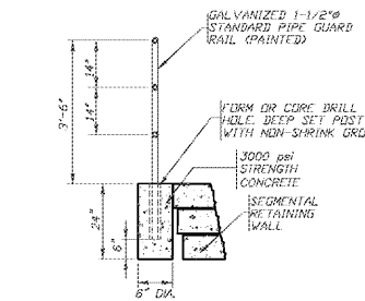
6 C7.0 DETAIL: PIPE GUARD RAIL AT S.R.W. (NTS)
