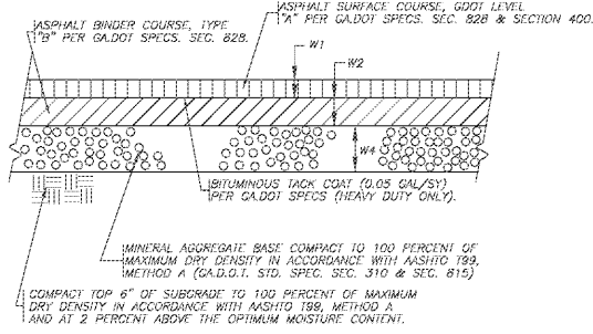
1 C7.0 DETAIL: ASPHALT PAVEMENT SECTIONS (NTS)
