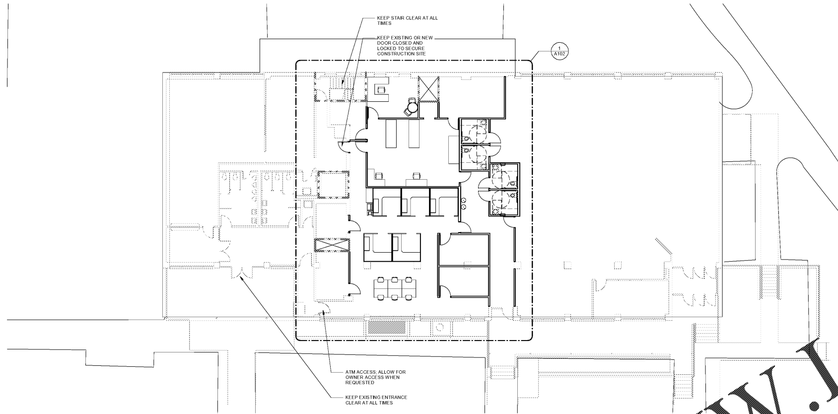
1 OVERALL PLAN 1" = 10'-0"
