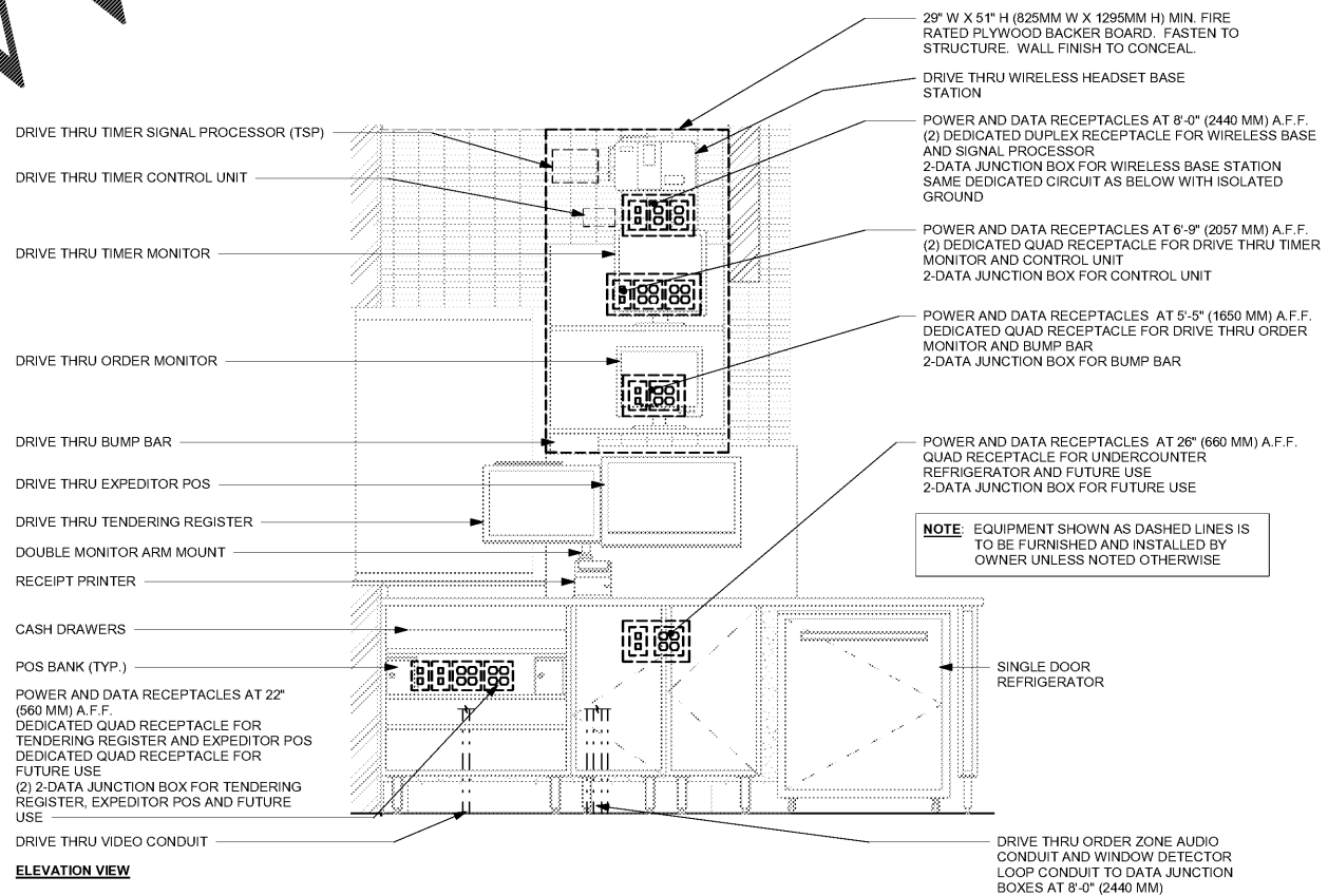
4 DRIVE - THRU POS DIAGRAM FOR REFERENCE ONLY
