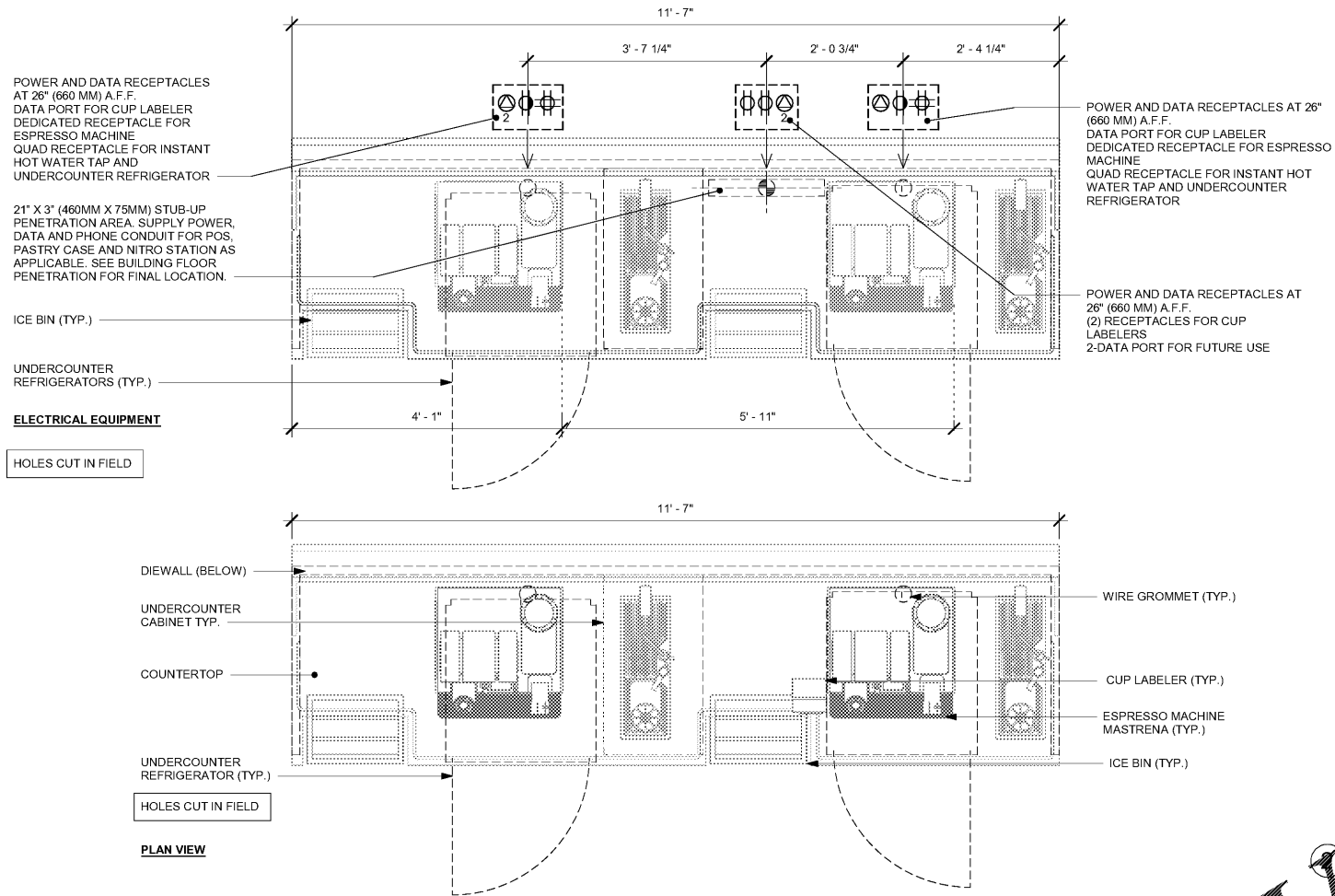
1 ESPRESSO - ELECTRICAL FOR REFERENCE ONLY
