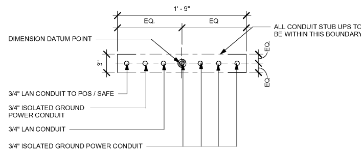
2 STUB UPS - FRONTBAR
