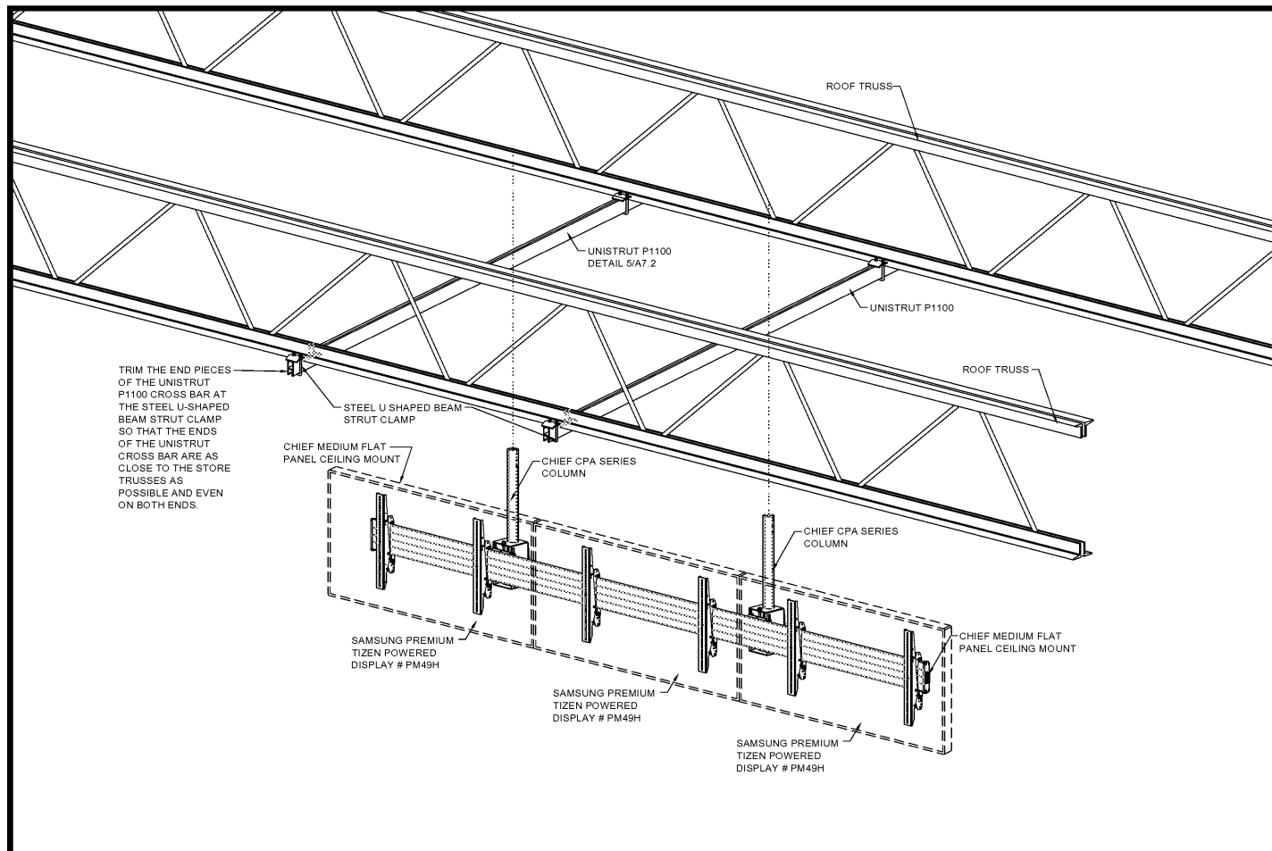
① GENERAL THREE MENU BOARDS/PROMO SCREEN CEILING MOUNTING DETAIL
