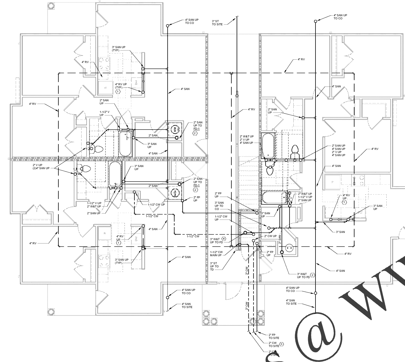
1 PLUMBING UNDERSLAB FLOOR PLAN - BUILDING I-C 1/4" = 1'-0"
