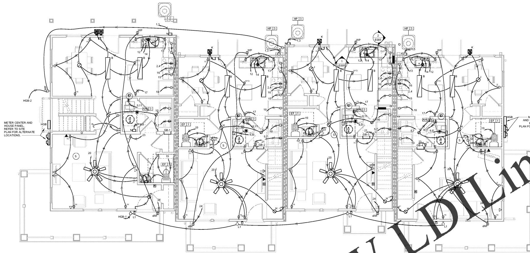
1 ELECTRICAL GROUND FLOOR PLAN - BUILDING G-B 1/4" = 1'-0"
