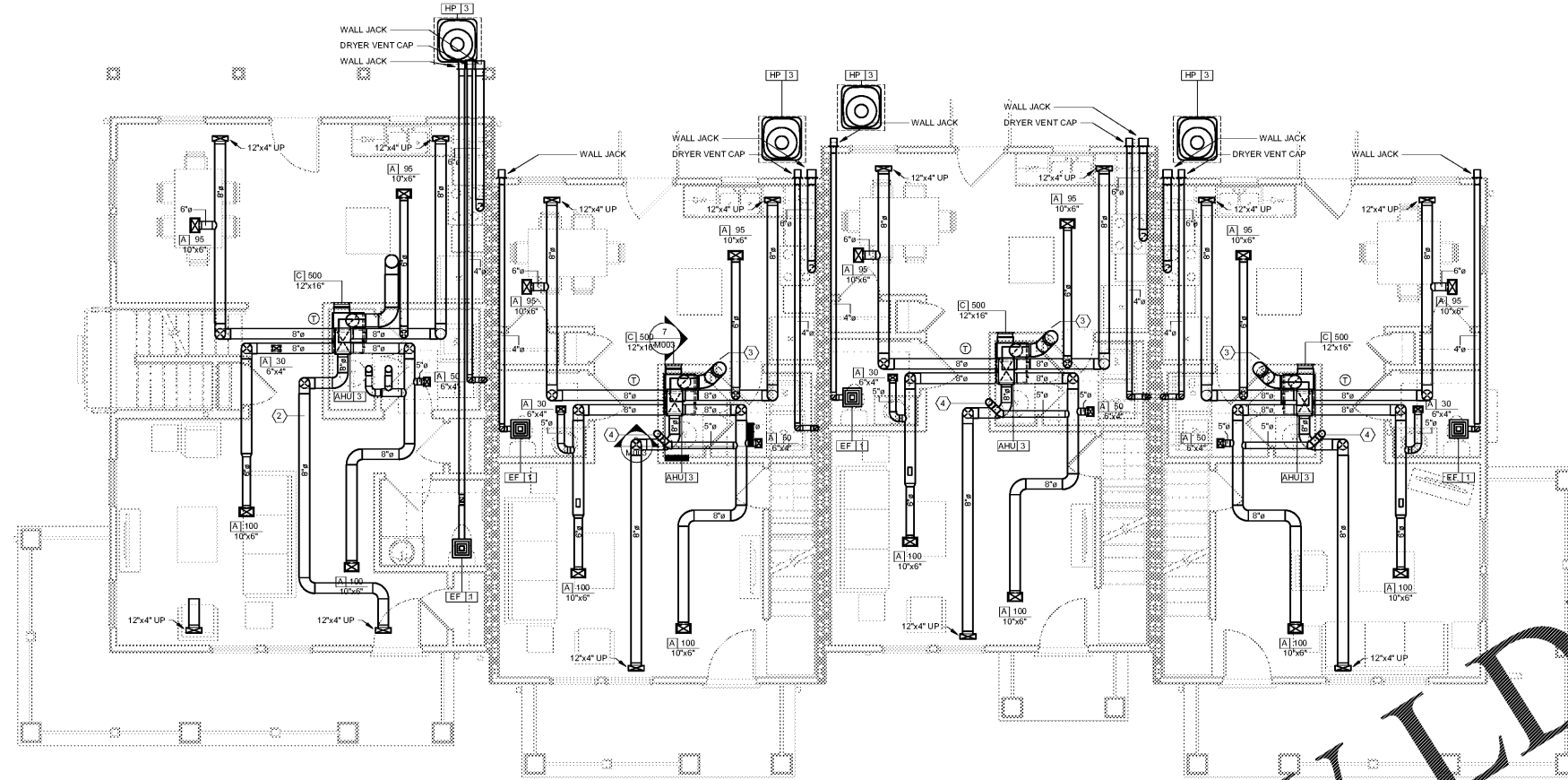
1 MECHANICAL GROUND FLOOR PLAN - BUILDING G-B 1/4" = 1'-0"
