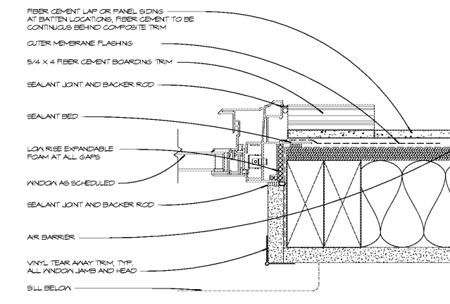
29 WINDOW JAMB AT FIBER CEMENT
