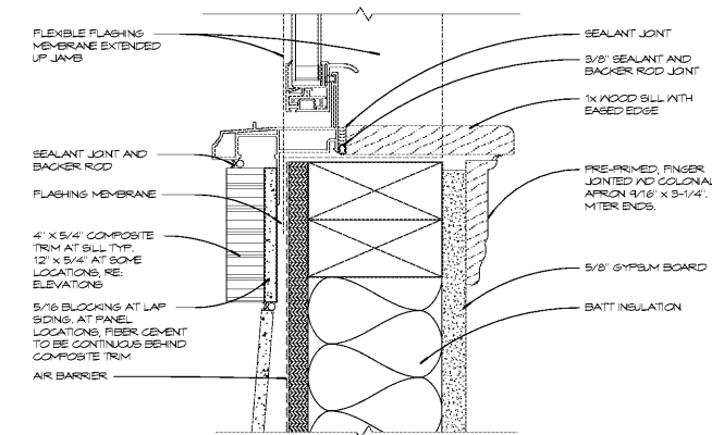
23 WINDOW SILL AT FIBER CEMENT
