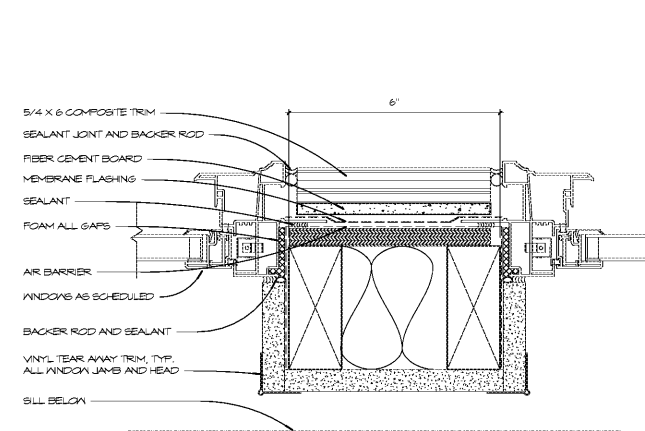
25 WINDOW JAMB GANGED WINDOW
