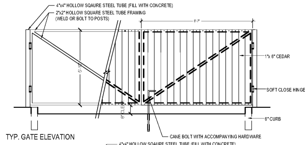
TYP. GATE ELEVATION
