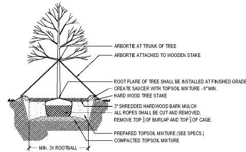
1 TYPICAL DECIDUOUS TREE PLANTING
