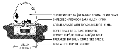
1 TYPICAL DECIDUOUS TREE PLANTING
