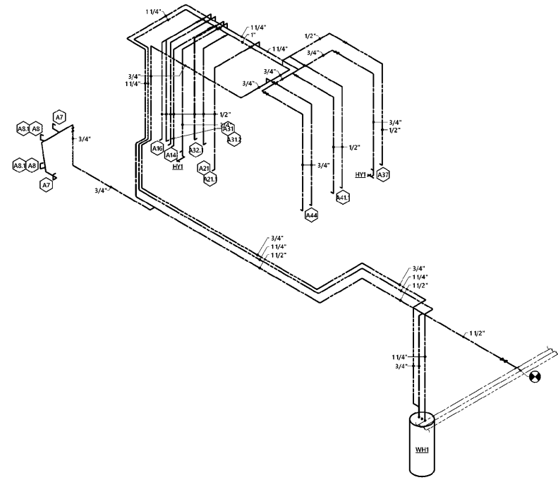
3 PLUMBING RISER DIAGRAM - WATER SUPPLY NOT TO SCALE
