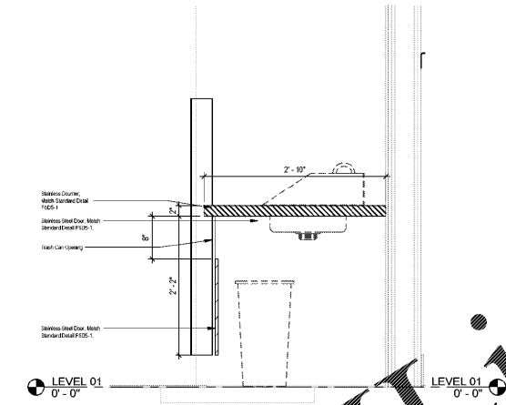
② Back Counter Section at Hand Sink SCALE: 1" = 1'-0"
