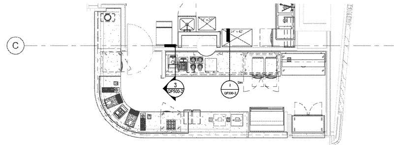
① Foodservice Counter Section Plan SCALE: 1/4" = 1'-0"
