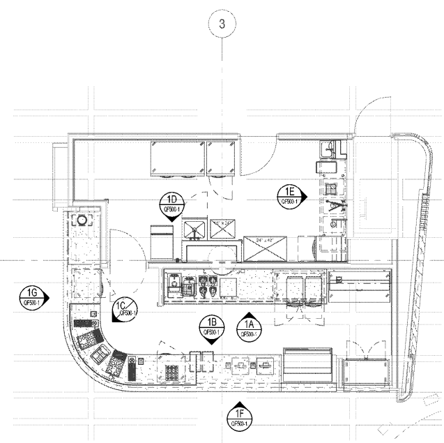
1 Foodservice Elevation Plan SCALE: 1/4" = 1'-0"
