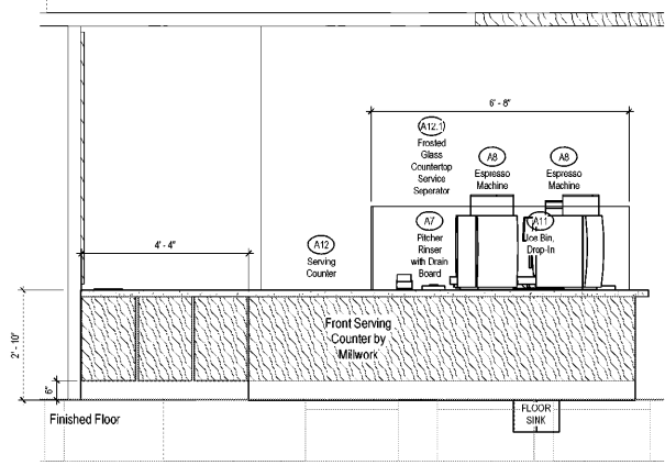
1G Serving Counter Coffee Customer Side SCALE: 1/2" = 1'-0"
