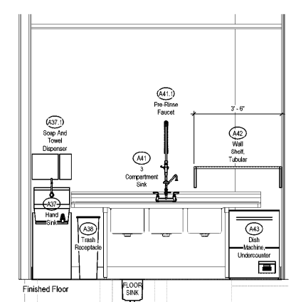
1E Three Compartment Sink SCALE: 1/2" = 1'-0"
