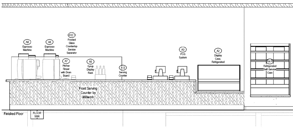
1F Serving Counter Pickup Customer Side SCALE: 1/2" = 1'-0"
