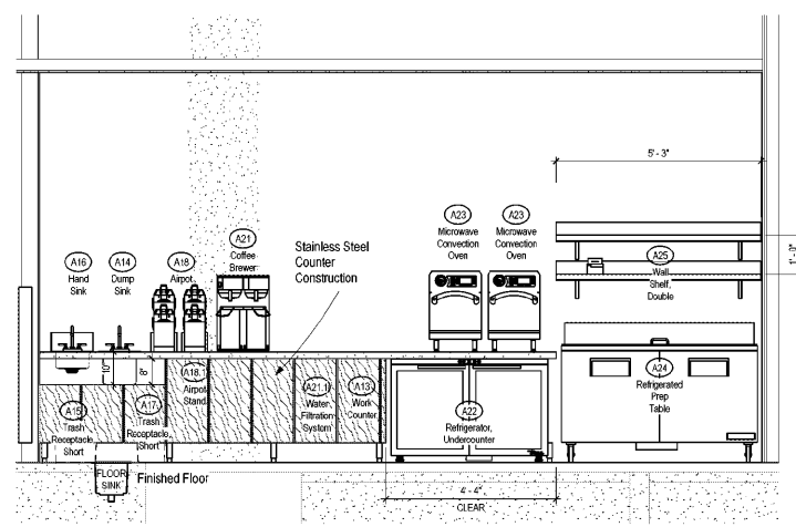
1A Work Counter SCALE: 1/2" = 1'-0"
