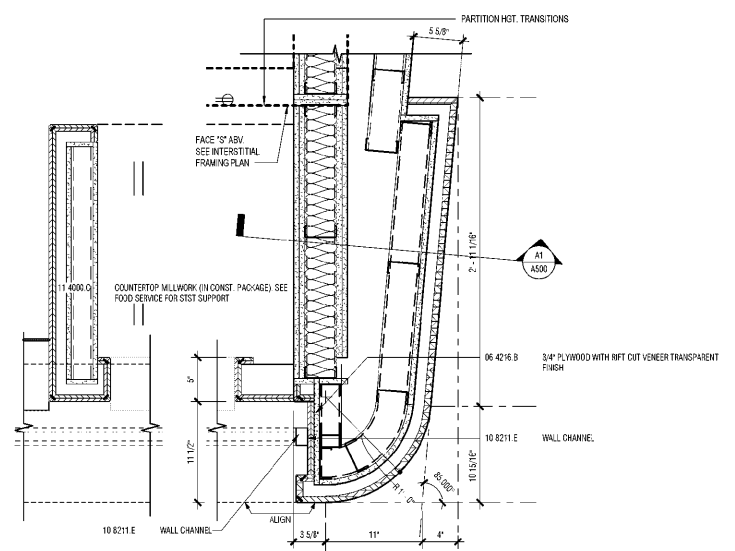
CS A411 ENLARGED PLAN - SELF-SERVICE COOLER & WD. WALL @ CAFE 1 1/2" = 1'-0"
