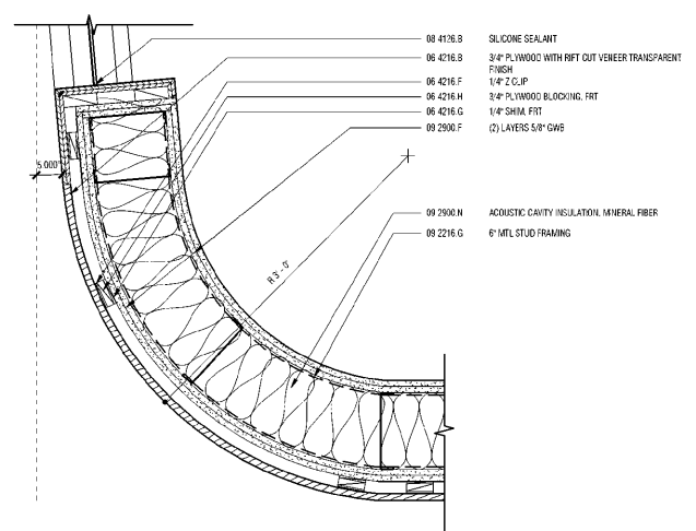
AS A411 ENLARGED PLAN - LIBRARY WALL 1 1/2" = 1'-0"
