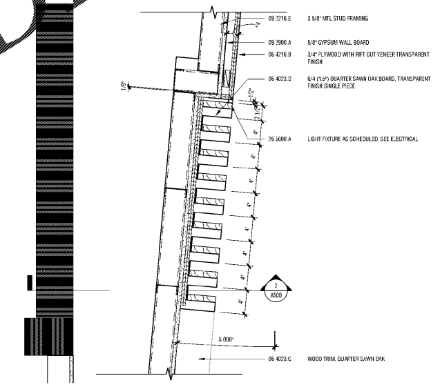
BS A411 ENLARGED PLAN - WD. SCREEN @ EAST WALL 1 1/2" = 1'-0"
