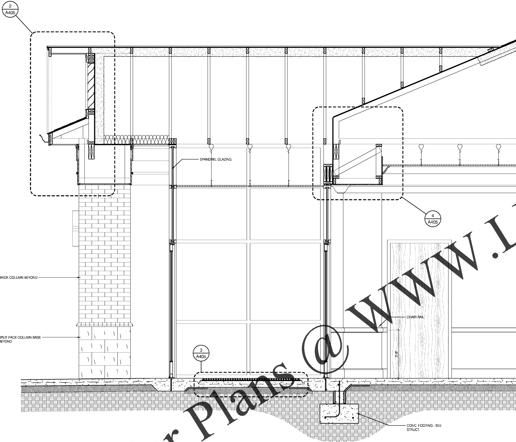
1 SECTION THRU MAIN ENTRY 3/4" = 1'-0"
