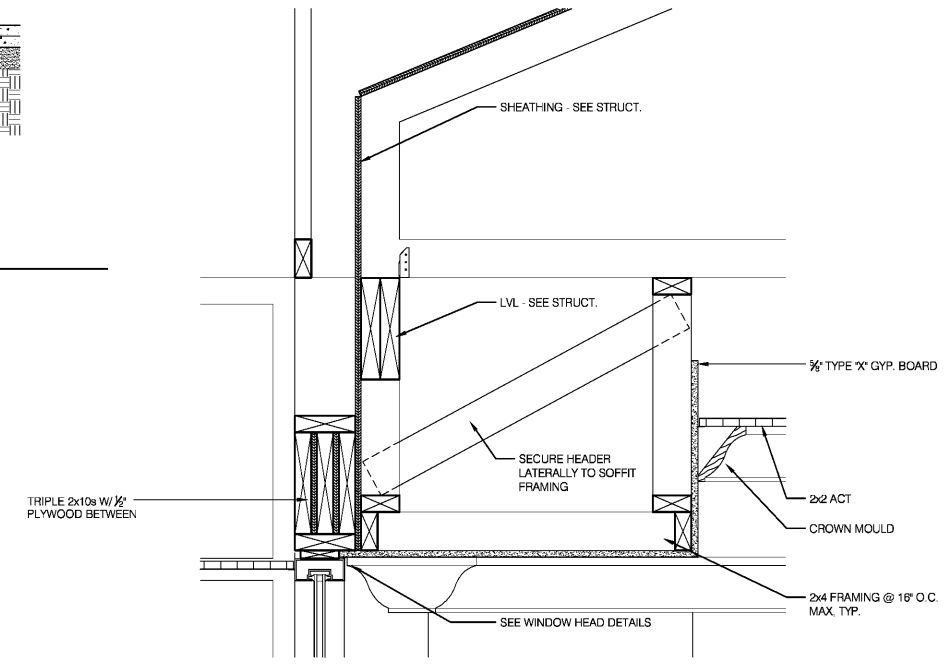
4 DETAIL @ ENTRY 1 1/2" = 1'-0"
