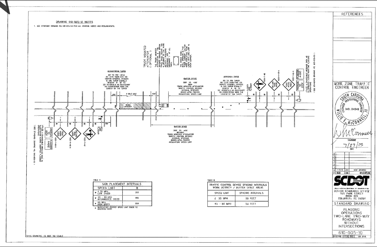
TYPICAL SCDOT FLAGGING OPERATIONS DETAIL FOR 2-LANE 2-WAY ROADWAYS NOT TO SCALE
