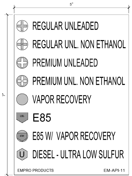
1 VARIOUS COLORED LETTERING WITH WHITE BACKGROUND SCALE: 1'-0" = 1'-0"
