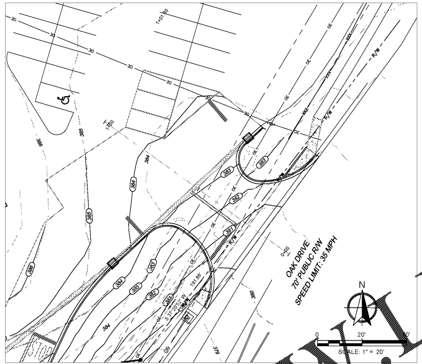
DRIVEWAY PLAN
