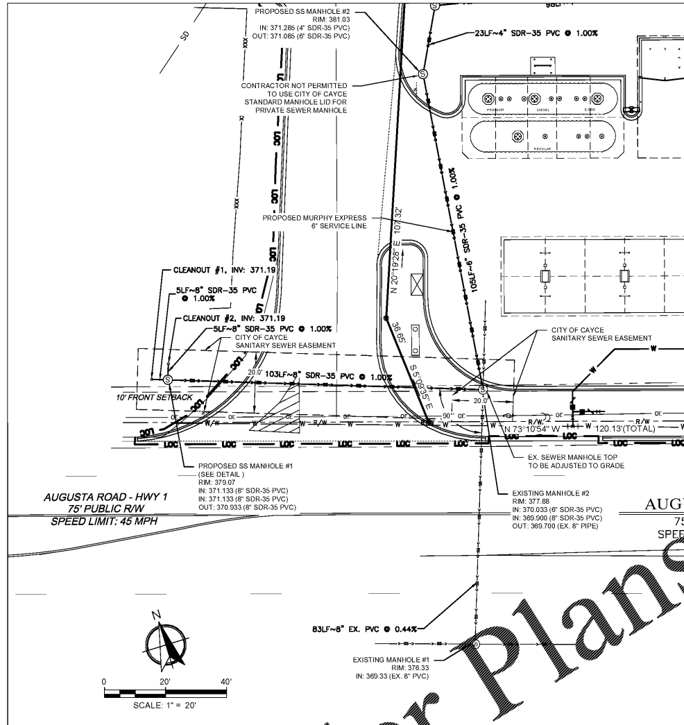
SANITARY SEWER PLAN
