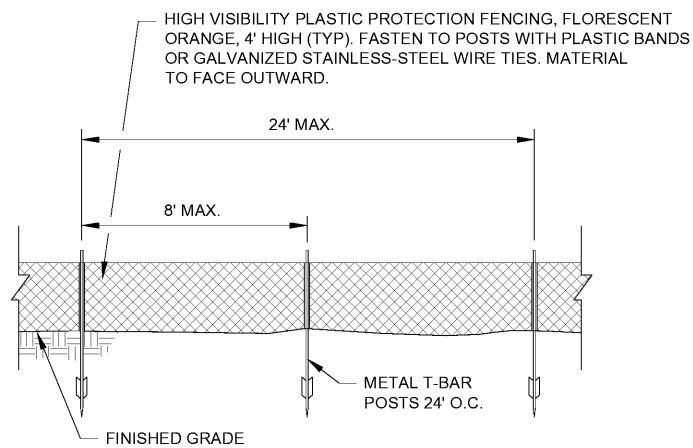
4 TREE PROTECTION FENCING DETAIL C7.02 SCALE: NTS
