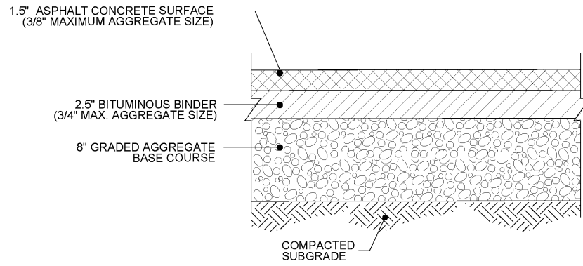
2 HEAVY DUTY ASPHALT PAVING SECTION C7.02 SCALE: NTS
