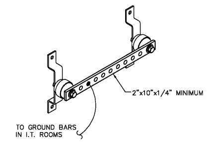
INTERSYSTEM GROUND BAR DETAIL SCALE: NONE
