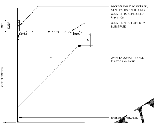
C3 BASE - COUNTER / KNEE SPACE 1 1/2\"/>
