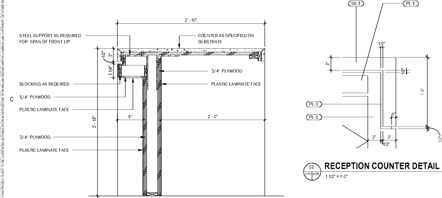
C1 RECEPTION AT KNEE SPACE 1 1/2\"/>
