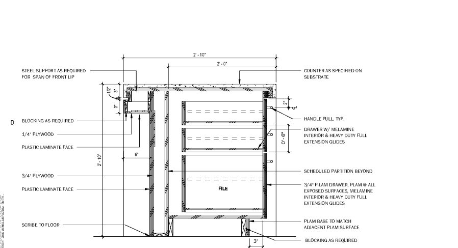
D1 RECEPTION AT DRAWERS 1 1/2\"/>
