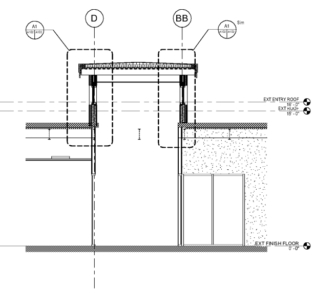
C1 A102 SECTION - CLERESTORY 1 1/2" x 1'-0"
