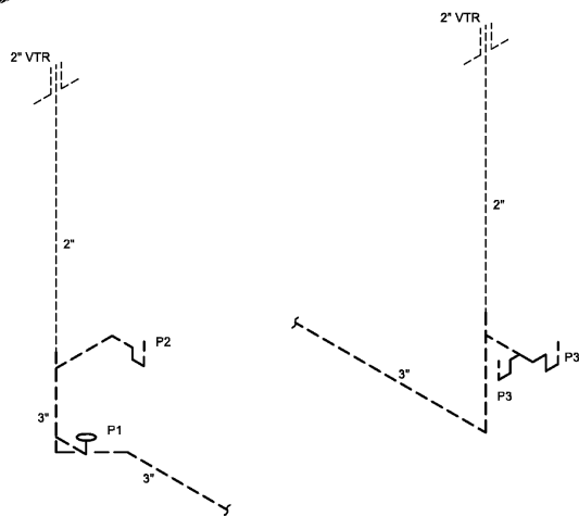
2 WASTE & VENT RISER DIAGRAM P-2.0 SCALE: NONE
