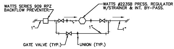
PRESSURE REDUCING STATION DETAIL NOT TO SCALE
