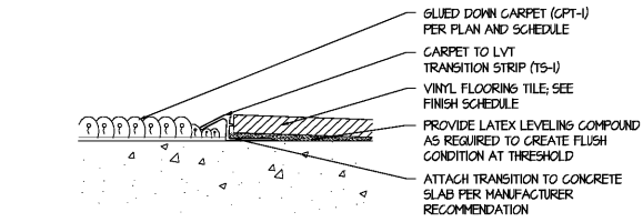
2 CPT to LVT Transition Scale: NTS
