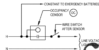
TOILET ROOM OCCUPANCY CONTROL SCHEME N.T.S.
