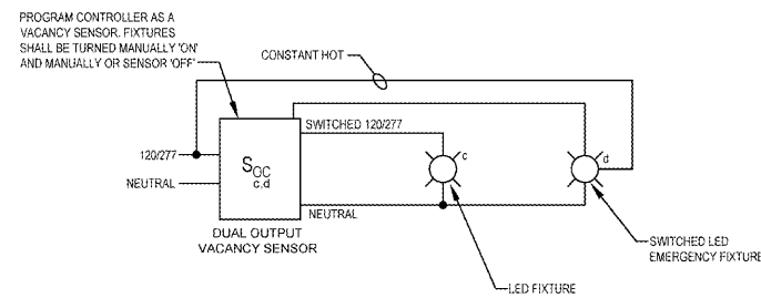
CASH ROOM CONTROL SCHEME N.T.S.
