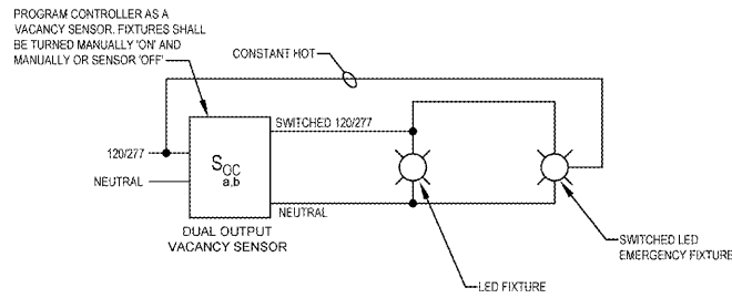
MANAGER'S OFFICE CONTROL SCHEME N.T.S.
