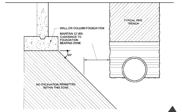
9 DETAIL - PIPE TRENCH LOCATION P5.02 N.T.S.
