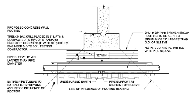
7 DETAIL - FOUNDATION WALL SLEEVE P5.02 N.T.S.
