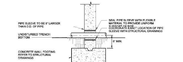
8 DETAIL - FOUNDATION WALL PIPE SLEEVE P5.02 N.T.S.
