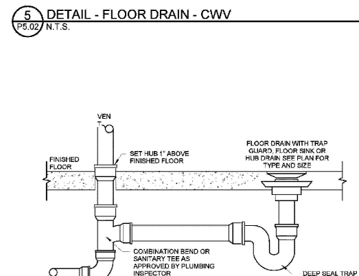
5 DETAIL - FLOOR DRAIN - CWV P5.02 N.T.S.
