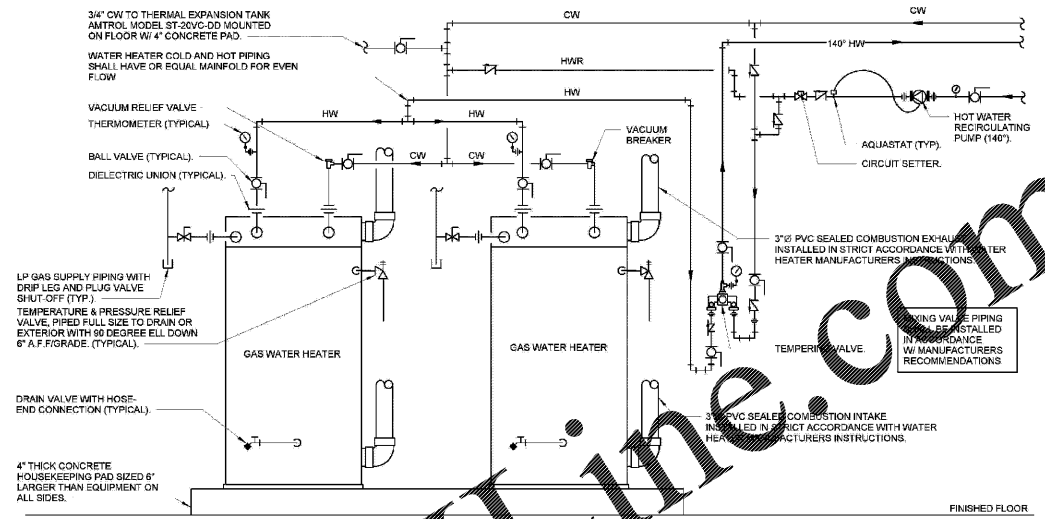
1 DETAIL - WATER HEATER - GAS FIRED - INSTANTANEOUS P5.02 N.T.S.
