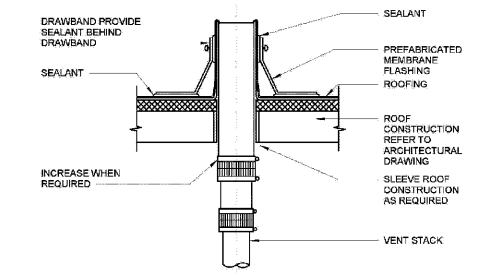
7 DETAIL - VENT THROUGH ROOF (VTR) P5.01 N.T.S.
