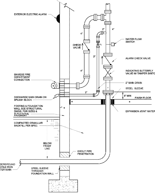
2 DETAIL - FIRE PROTECTION SERVICE ENTRANCE P5.01 N.T.S.
