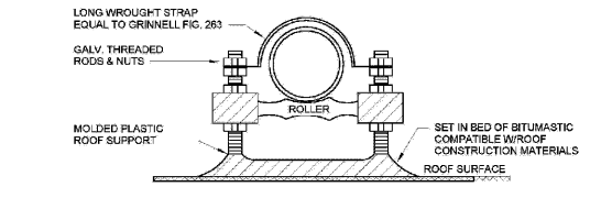
9 DETAIL - ROOF PIPE SUPPORT W/ ROLLER P5.01 N.T.S.
