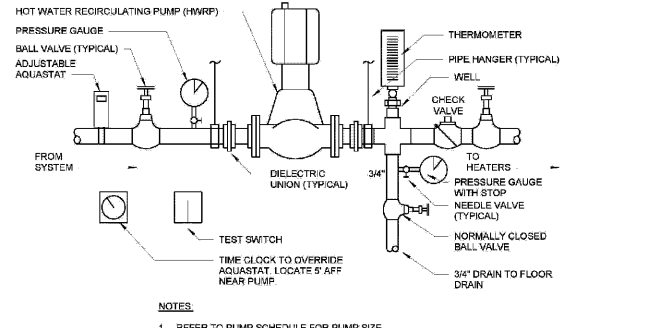
5 DETAIL - HOT WATER RECIRCULATING PUMP (HWRP) P5.01 N.T.S.
