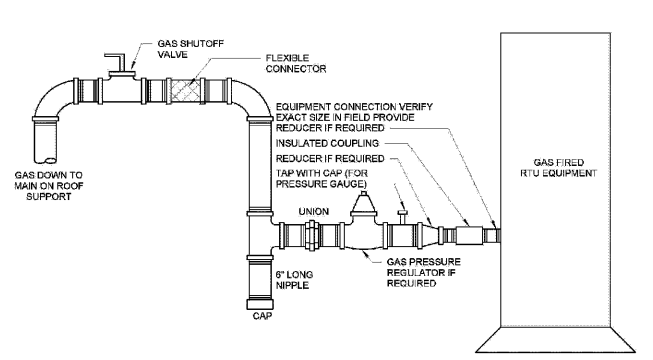
6 DETAIL - EXTERIOR GAS FIRED EQUIPMENT CONNECTION P5.01 N.T.S.
