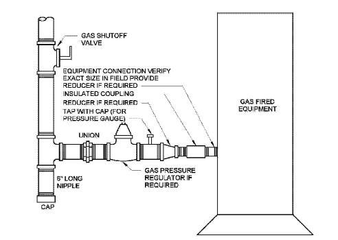
3 DETAIL - GAS FIRED EQUIPMENT CONNECTION P5.01 N.T.S.
