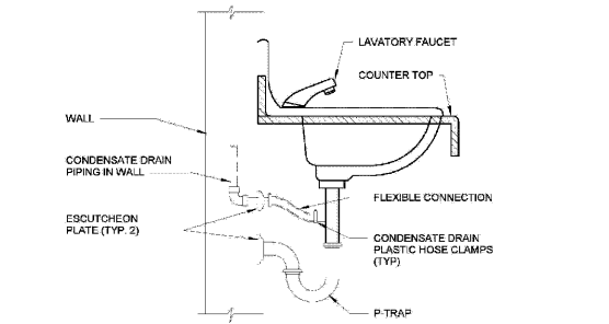
3 CONDENSATE DRAIN TO LAVATORY TAILPIECE DETAIL M4.01 N.T.S.
