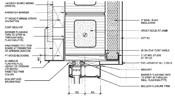
07 DECK BOARD SIDING WALL WINDOW SYSTEM JAMB 3\"/>
