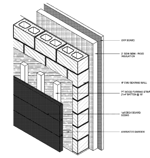
01 DECK BOARD SIDING WALL SYSTEM 3\"/>
