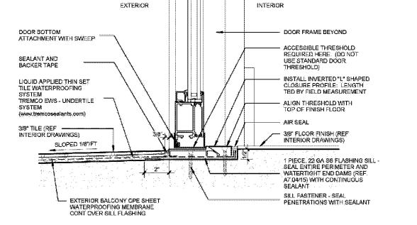
04 OUT-SWING DOOR PANEL ACCESSIBLE THRESHOLD 3\"/>
