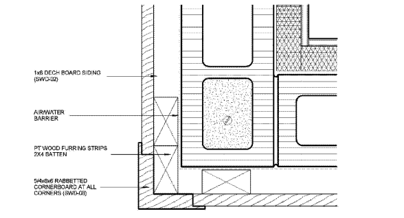
05 DECK BOARD SIDING CORNER DETAIL 3\"/>
