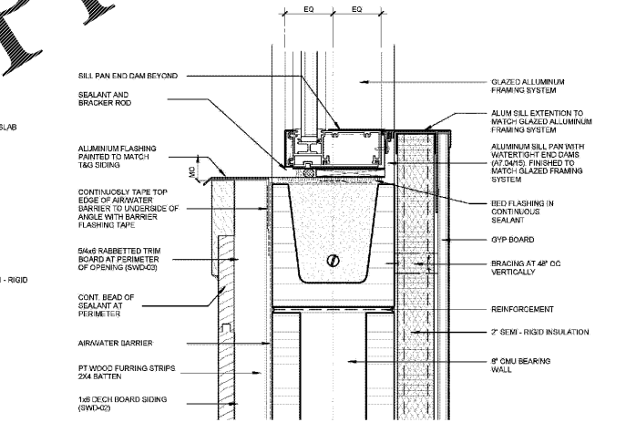
08 DECK BOARD SIDING WALL WINDOW SYSTEM SILL 3\"/>
