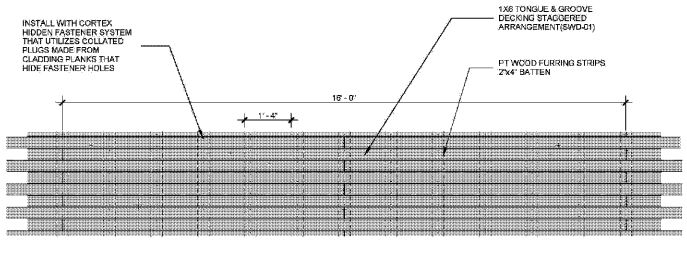
11 T&G TYPICAL LAYOUT 1/2\"/>
