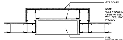
14 FRAMING AT 1-HR WALL FIRE EXTINGUISHER CABINET AT RATED WALL 1 1/2" = 1'-0"
