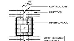
01 CONTROL JOINT AT FIRE-RATED PARTITION 3" = 1'-0"
