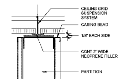
03 CONTROL JOINT AT PARTITION ATTACHMENT TO CEILING GRID 3" = 1'-0"
