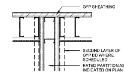
09 INTERSECTION AT RATED PARTITION AT EXTERIOR WALL 3" = 1'-0"
