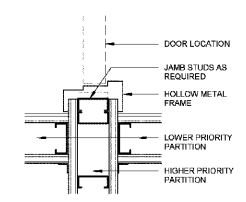
13 INTERSECTION AT CROSS CORRIDOR DOOR ONE HOUR RATED PARTITION 3" = 1'-0"
