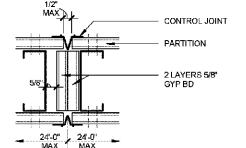
08 CONTROL JOINT AT FIRE-RATED PARTITION 3" = 1'-0"
