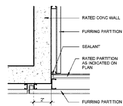
11 INTERSECTION AT RATED PARTITION AT CONCRETE WALL 3" = 1'-0"
