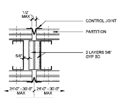
07 CONTROL JOINT AT FIRE-RATED PARTITION 3" = 1'-0"
