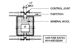
02 CONTROL JOINT AT FIRE-RATED PARTITION 3" = 1'-0"
