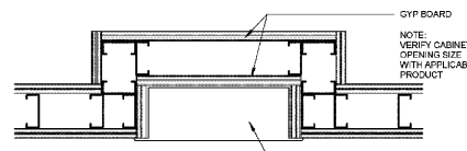
15 FRAMING AT 2-HR WALL FIRE EXTINGUISHER CABINET AT RATED WALL 1 1/2" = 1'-0"
