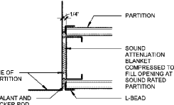
05 CONTROL JOINT AT PARTITION INTERSECTION CHANGE IN CONSTRUCTION 3" = 1'-0"
