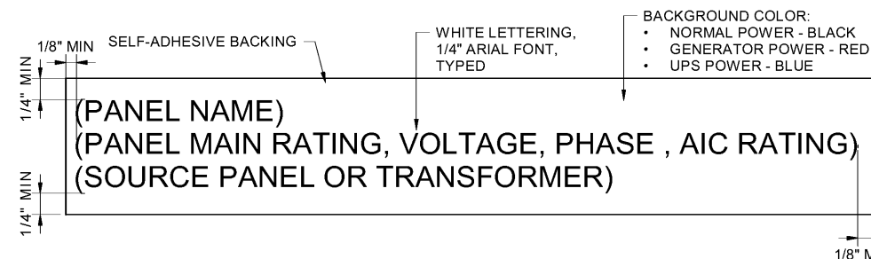
A3 PANELBOARD LABEL
