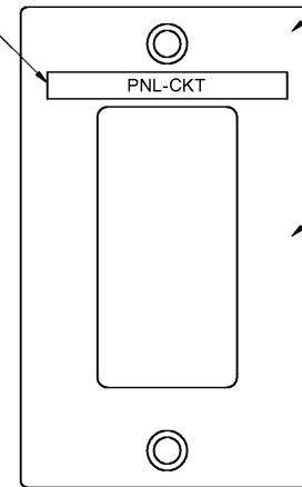
C2 LIGHT SWITCH DETAIL (TYP.)
