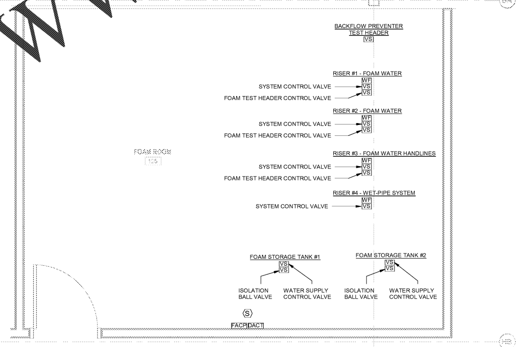
A3 FIRE ALARM PLAN - FOAM ROOM SCALE: 1/2" = 1'-0"
