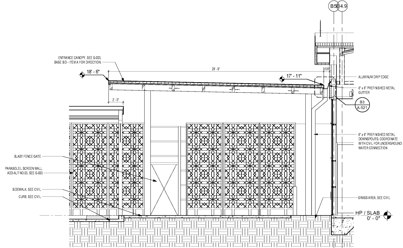
C1 CANOPY SECTION EAST TO WEST SCALE: 1/4" = 1'-0"
