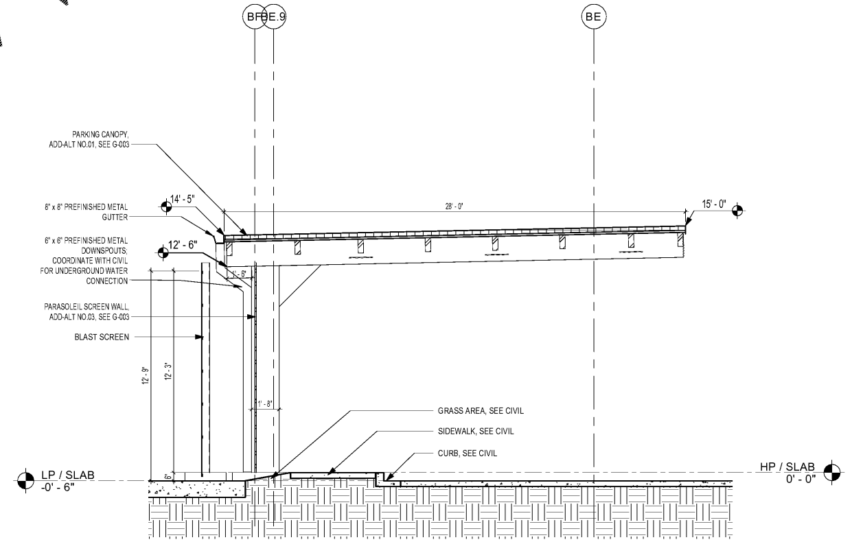
A4 CANOPY SECTION NORTH TO SOUTH SCALE: 1/4" = 1'-0"
