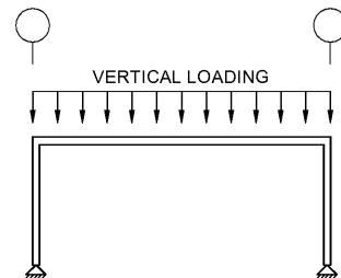
CANOPY GRAVITY LOADING
