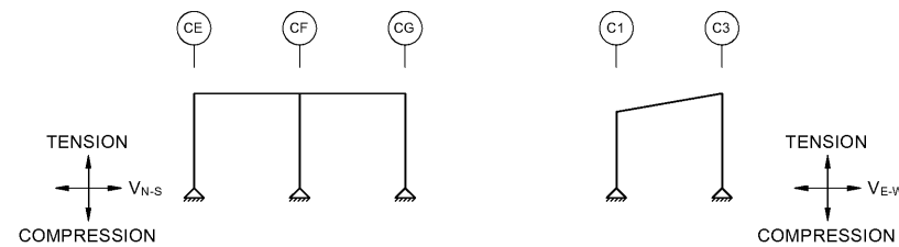
DESIGN BASE REACTIONS
