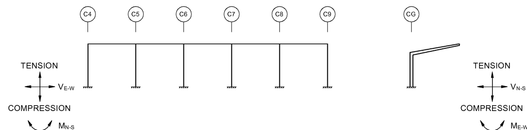
DESIGN BASE REACTIONS
