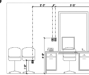
14 MANAGER'S OFFICE SCALE: 1/2" = 1'-0"
