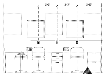
16 DEPT. MANAGER'S OFFICE SCALE: 1/2" = 1'-0"
