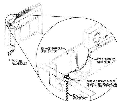
CUSTOMER SERVICE SIGNAGE ELECTRICAL DETAIL
