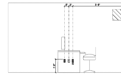
15 MANAGER'S OFFICE SCALE: 1/2" = 1'-0"
