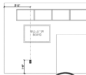
12 MANAGER'S OFFICE SCALE: 1/2" = 1'-0"
