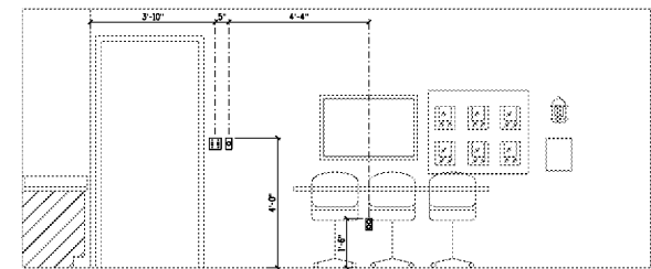
7 GENERAL OFFICE SCALE: 1/2" = 1'-0"
