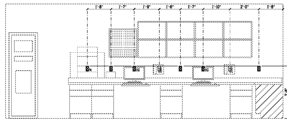
5 GENERAL OFFICE SCALE: 1/2" = 1'-0"
