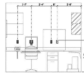
18 DEPT. MANAGER'S OFFICE SCALE: 1/2" = 1'-0"
