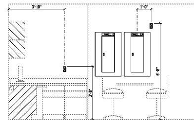
6 GENERAL OFFICE SCALE: 1/2" = 1'-0"
